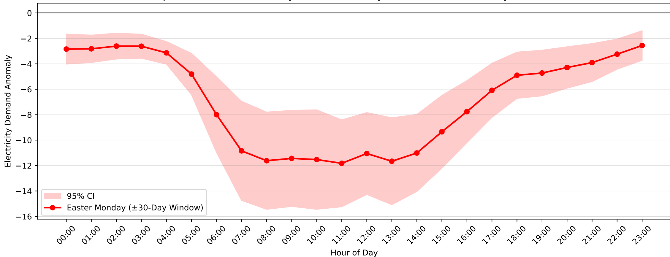
Milperra Demand Anomaly: Easter Monday (2004-2017, \pm 30 -Day Window)
